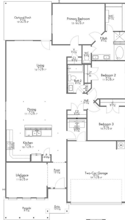
Building Envelope 48'-0" x 39'-3"
