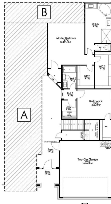
Building Envelope 70'-1 1/2" x 29'-1 1/2"
